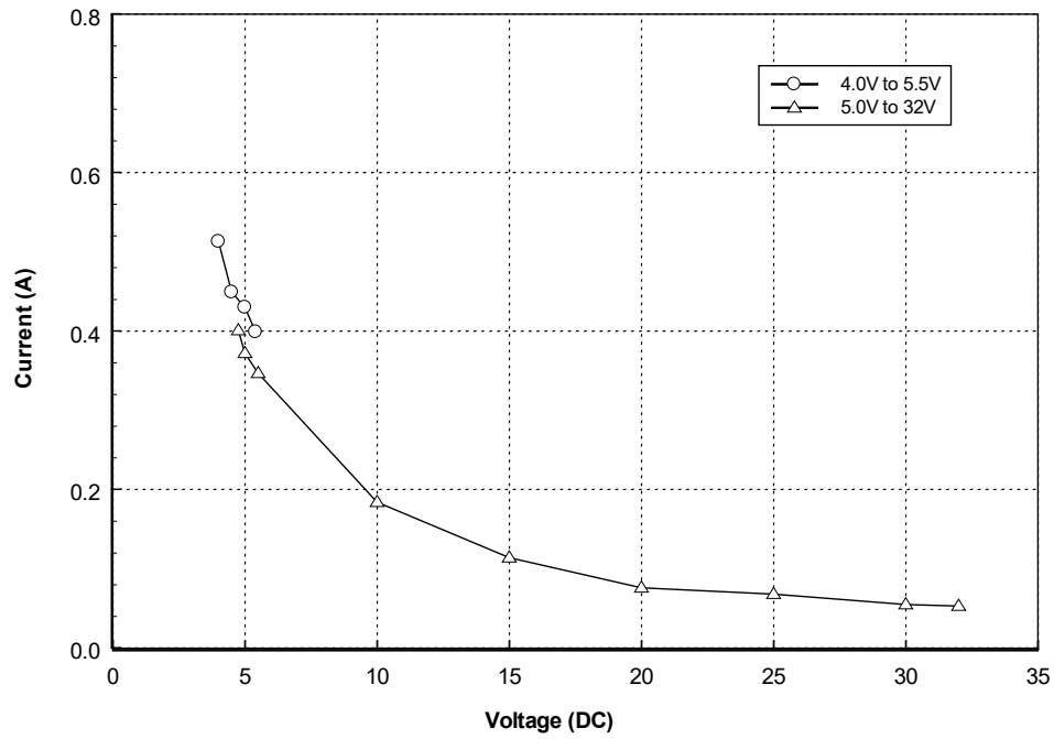
Figure 10: Average Current Drawn During a Data Switch Call
