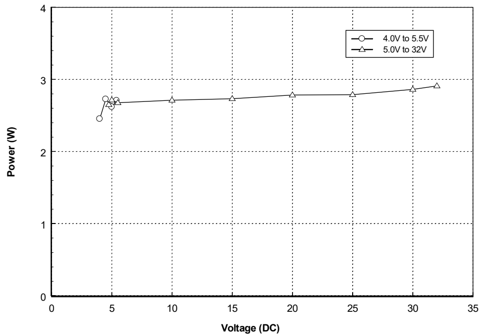
Figure 9: Average Power Consumption During Standby with DPL Handset
