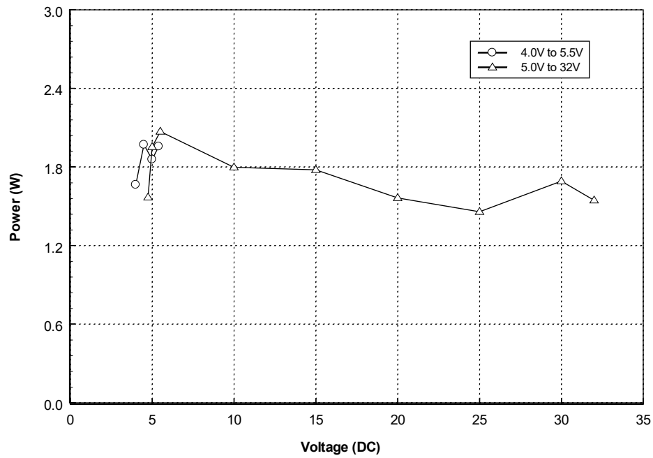
Figure 15: Average Power Consumption During an SMS Transmission
