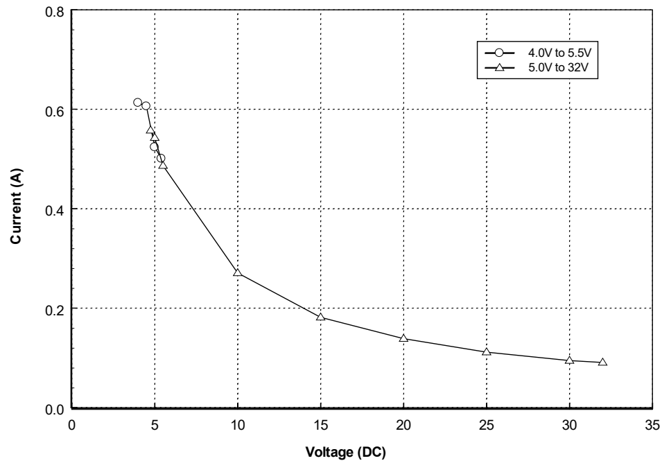
Figure 8: Average Current Drawn During Standby with DPL Handset
