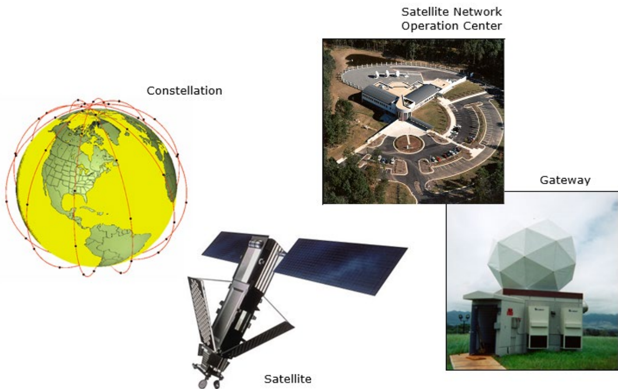
Figure 18: Iridium Network Major Components
