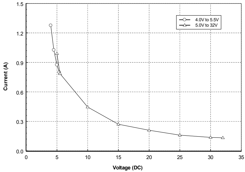
Figure 16: Average Current Drawn During a Voice Call Using DPL Handset
