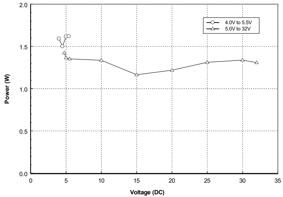
Figure 13: Average Power Consumption During an SBD Transmission
